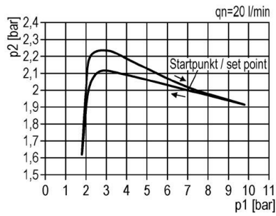
pressure characteristic
